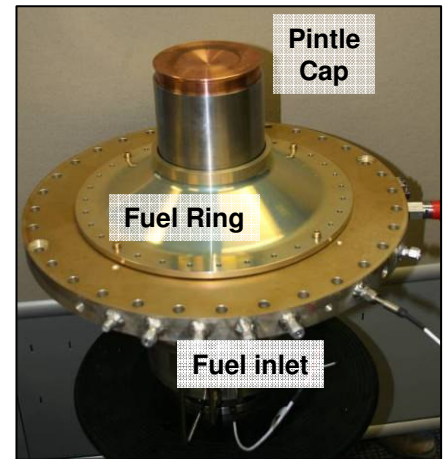
Injector
