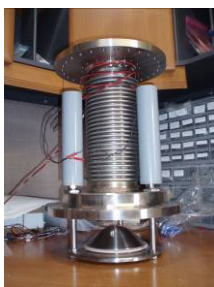
Isolation Valve, Full assembly (shown upside down)
